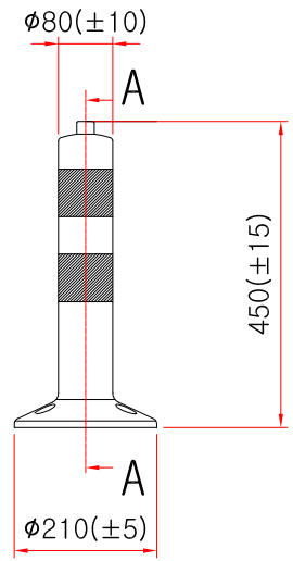
SIDE ELEVATION SCALE : NONE
